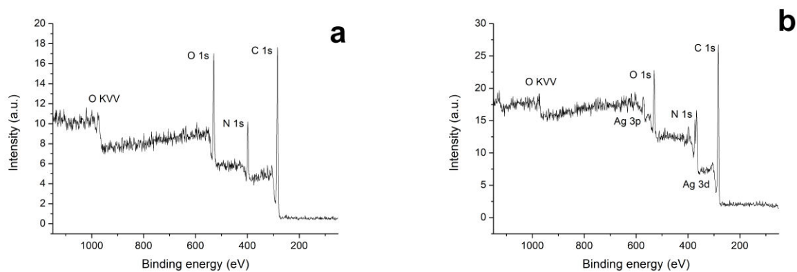
Figure S2. Full photoelectron spectra of the Col ( a ) and ColAgNPs ( b ) samples
