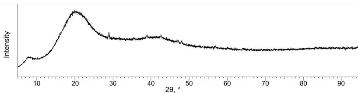
Figure S1. X-ray diffraction pattern of collagen
