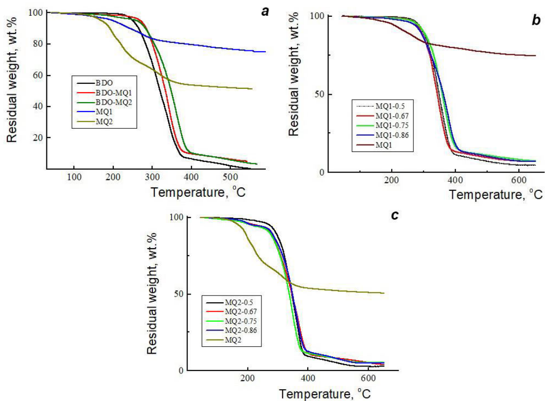
Fig. S1. Thermogravimetric curves of the PU obtained using different curing agents: BDO and mixtures BDO–MQ1, BDO–MQ2 (a); MQ1 (b) and MQ2 (c) at different resin concentrations
