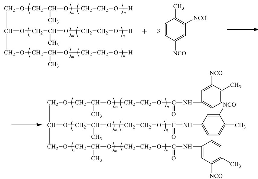
Fig. S2. Synthesis of the urethane prepolymer
