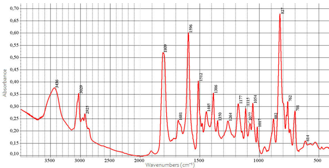
Figure S4. IR spectrum of P2 after saturation with CO 2 .
