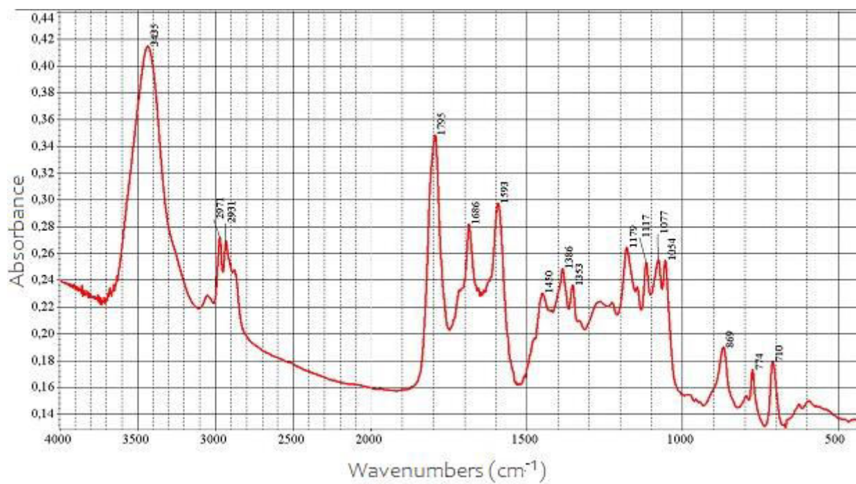
Figure S5. IR spectrum of P2 impregnated with compound 5 and saturated with CO 2 .
