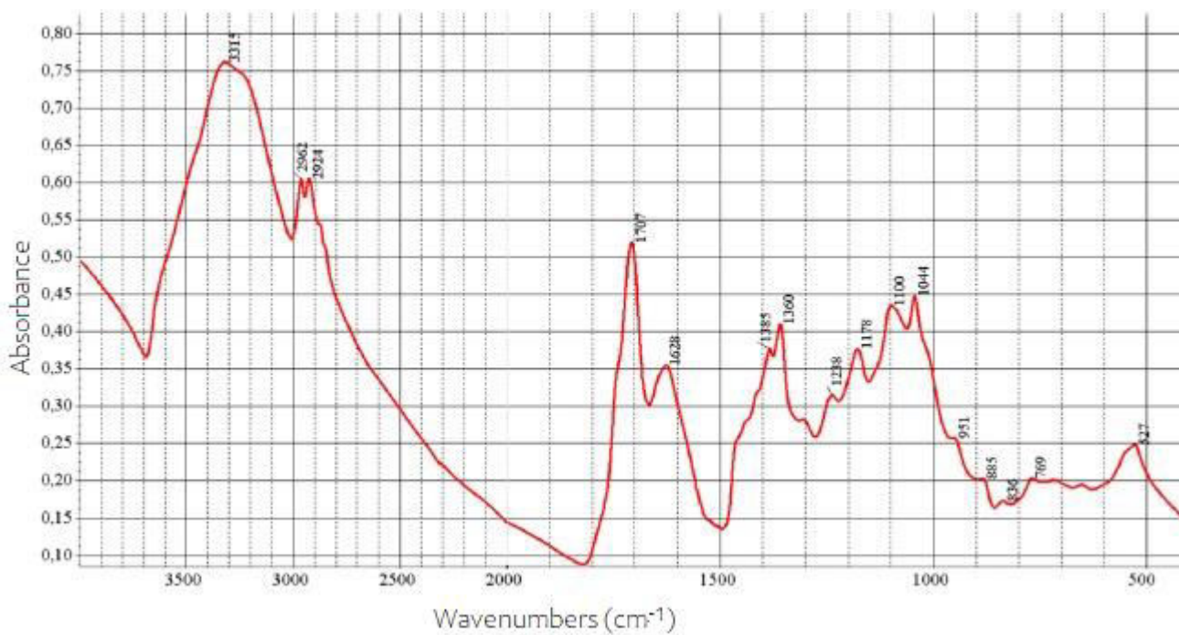
Figure S3. IR spectrum of compound 5.
