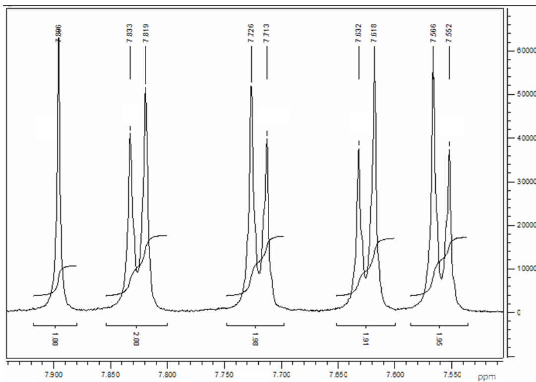
Figure S1. ^1\text{H} NMR spectrum of compound 3.
