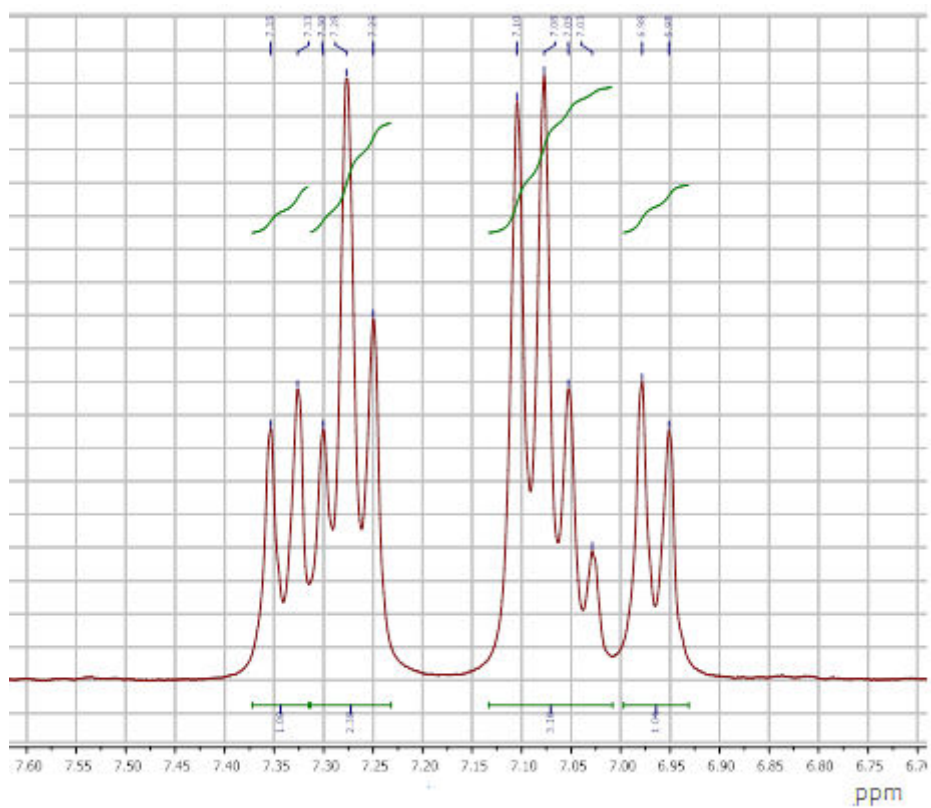
Figure S2. ^1\text{H} NMR spectrum of compound 4.
